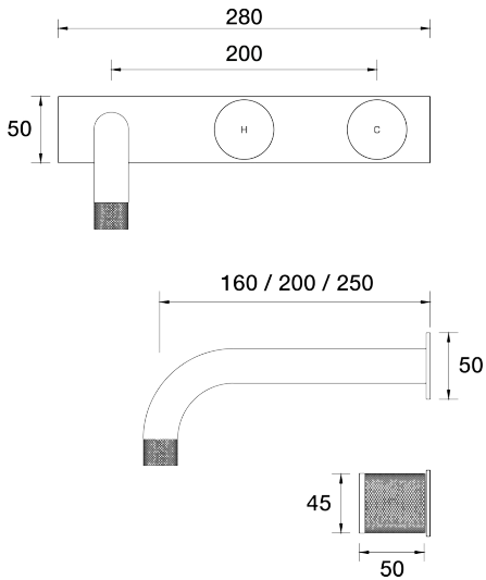
IDK Wall Bath Set 160mm Outlet on Plate - Offset B38.021.6.01 - Chrome
