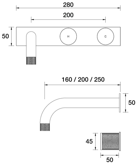
IDK Wall Bath Set 160mm Outlet on Plate - Offset B38.021.6.02 - Brushed Chrome
