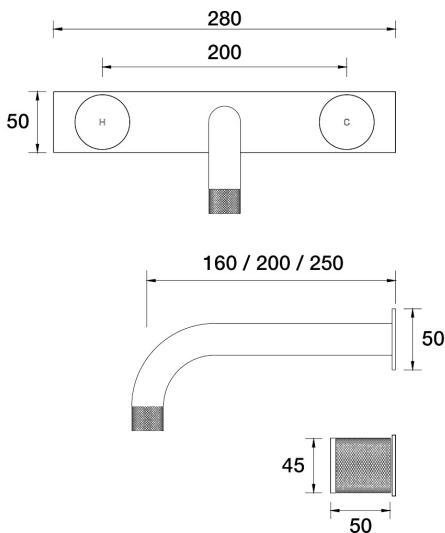
IDK Wall Bath Set 200mm Outlet on Plate B38.022.4.27 - Satin Pearl
