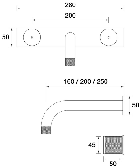
IDK Wall Bath Set 200mm Outlet on Plate B38.022.4.45 - Native Brass
