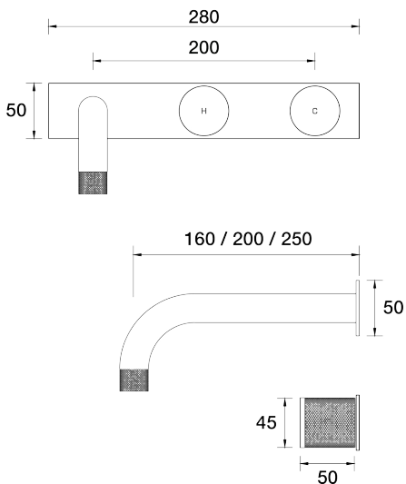
IDK Wall Bath Set 200mm Outlet on Plate - Offset B38.022.6.01 - Chrome
