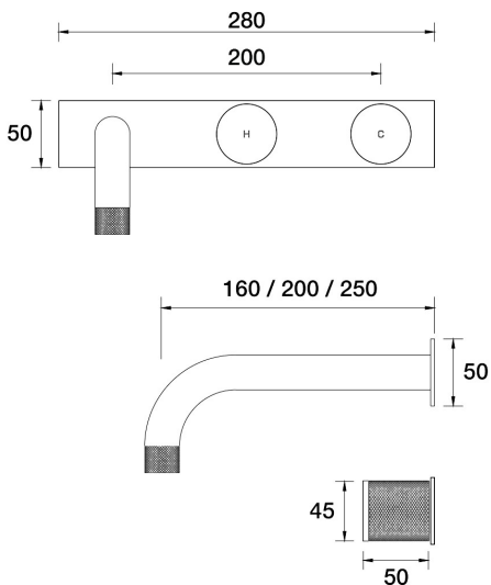
IDK Wall Bath Set 200mm Outlet on Plate - Offset B38.022.6.44 - Antique Copper
