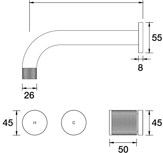
IDK Wall Bath Set 250mm Outlet B38.023.2.12 - 23k Brushed Gold
