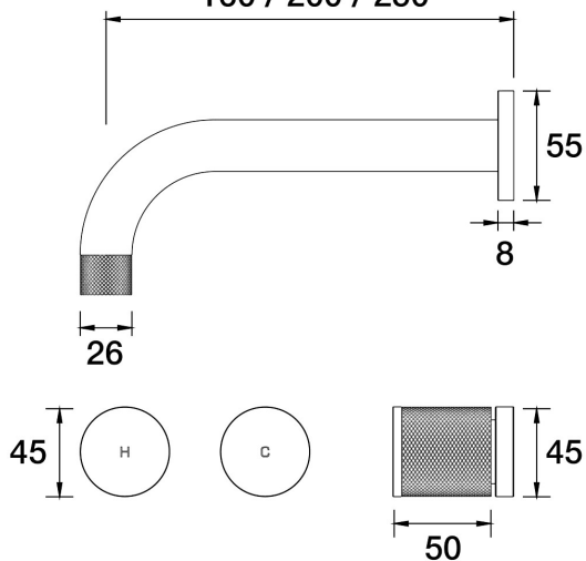
IDK Wall Bath Set 250mm Outlet B38.023.2.19 - 23k Brushed Brass Gold
