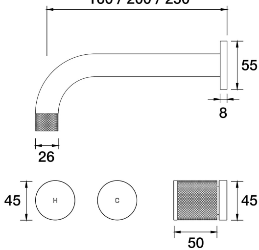
IDK Wall Bath Set 250mm Outlet B38.023.2.43 - Brass
