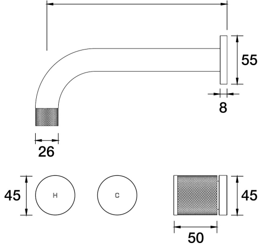
IDK Wall Bath Set 250mm Outlet B38.023.2.54 - Volcanic Grey
