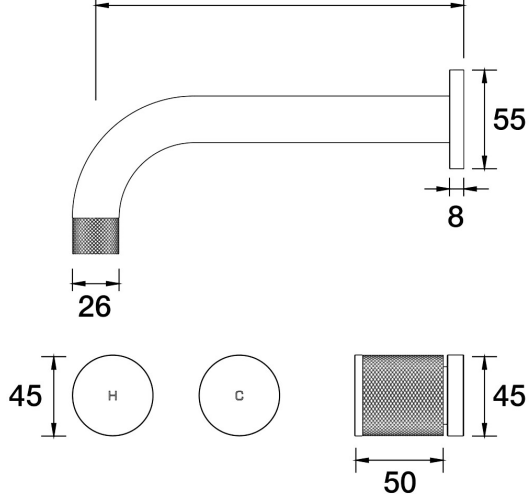
IDK Wall Bath Set 250mm Outlet B38.023.2.57 - Matt Nickel
