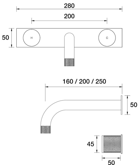
IDK Wall Bath Set 250mm Outlet on Plate B38.023.4.25 - Brushed Nickel
