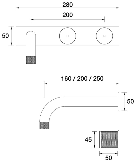
IDK Wall Bath Set 250mm Outlet on Plate - Offset B38.023.6.39 - Antique Bronze
