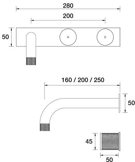
IDK Wall Bath Set 250mm Outlet on Plate - Offset B38.023.6.70 - Sea Spray
