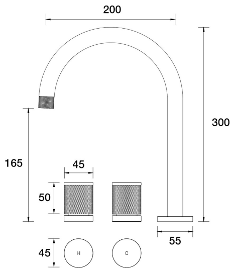
IDK Sink Set Hob Swivel B38.051.2.52 - Burnished
