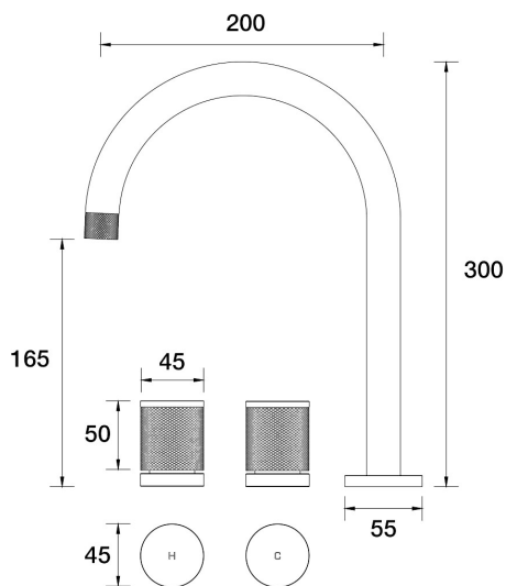
IDK Sink Set Hob Swivel B38.051.2.54 - Volcanic Grey
