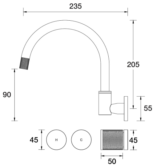
IDK Sink Set Wall Swivel B38.052.2.44 - Antique Copper
