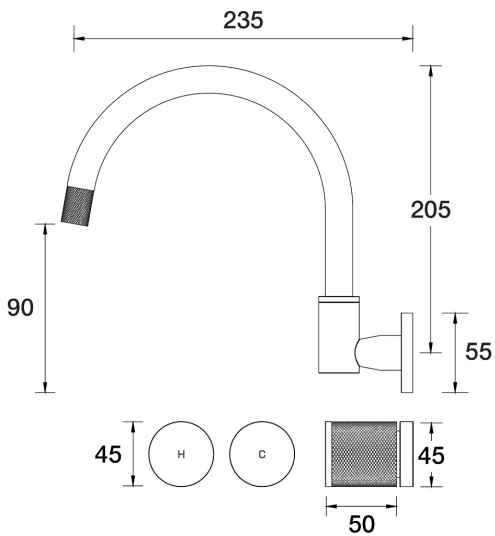
IDK Sink Set Wall Swivel B38.052.2.57 - Matt Nickel
