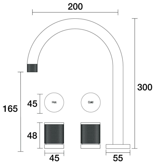
IDK Spa Set Hob Swivel B38.061.2.01 - Chrome
