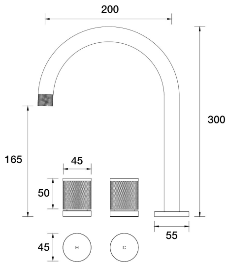
IDK Spa Set Hob Swivel B38.061.2.21 - Brushed Rose Gold
