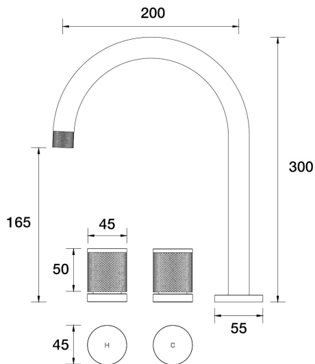
IDK Spa Set Hob Swivel B38.061.2.43 - Brass
