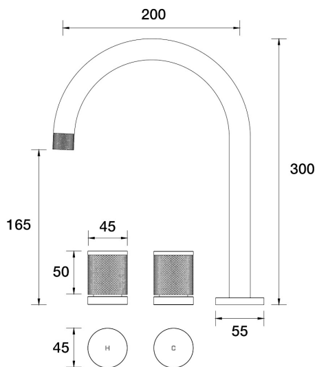
IDK Spa Set Hob Swivel B38.061.2.54 - Volcanic Grey
