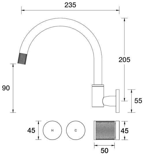
IDK Spa Set Wall Swivel B38.062.2.54 - Volcanic Grey
