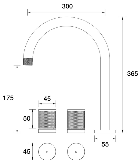
IDK Spa Set XL Hob Swivel B38.063.2.19 - 23k Brushed Brass Gold
