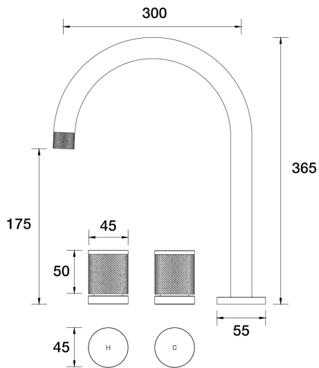
IDK Spa Set XL Hob Swivel B38.063.2.57 - Matt Nickel
