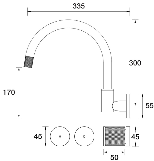
IDK Spa Set XL Wall Swivel B38.064.2.78 - Umber Earth
