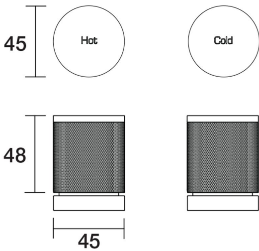
IDK Top Assemblies Wall Pair B38.082.2.01 - Chrome
