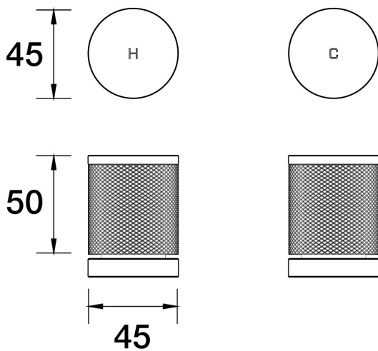
IDK Top Assemblies Wall Pair B38.082.2.41 - Brushed Brass
