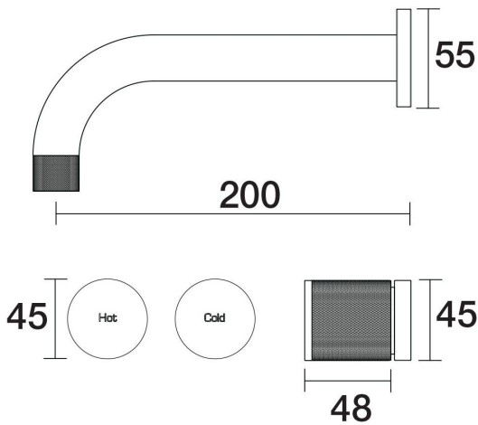
IDK Wall Basin Set Outlet 200mm B38.152.2.01 - Chrome
