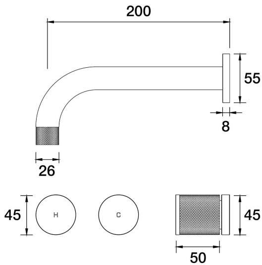
IDK Wall Basin Set Outlet 200mm B38.152.2.25 - Brushed Nickel
