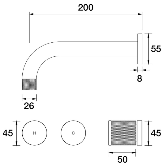
IDK Wall Basin Set Outlet 200mm B38.152.2.41 - Brushed Brass
