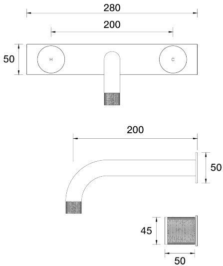
IDK Wall Basin Set Outlet 200mm on Plate B38.152.4.01 - Chrome
