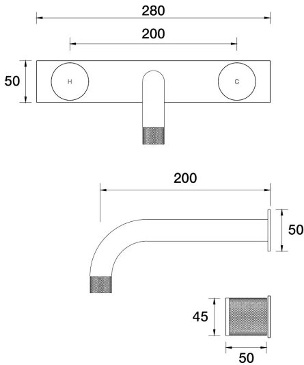
IDK Wall Basin Set Outlet 200mm on Plate B38.152.4.02 - Brushed Chrome
