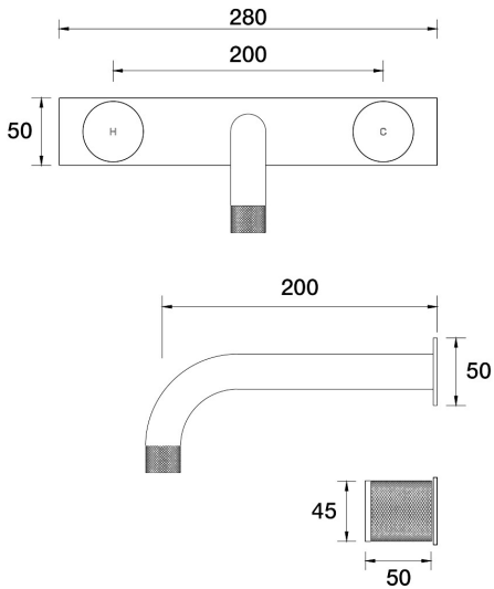
IDK Wall Basin Set Outlet 200mm on Plate B38.152.4.21 - Brushed Rose Gold
