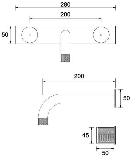
IDK Wall Basin Set Outlet 200mm on Plate B38.152.4.32 - Midnight Black
