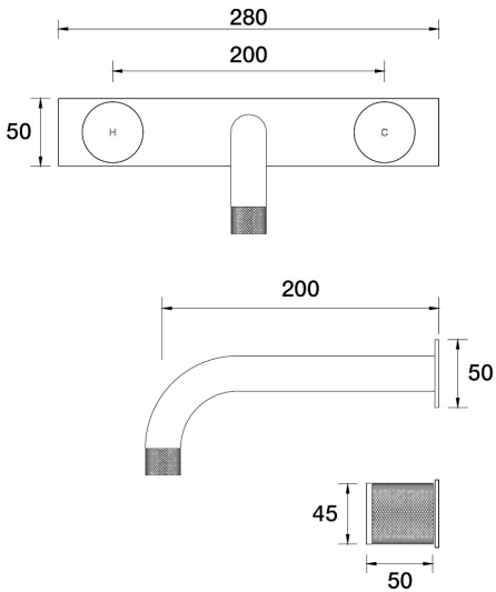
IDK Wall Basin Set Outlet 200mm on Plate B38.152.4.68 - Autumn Bronze
