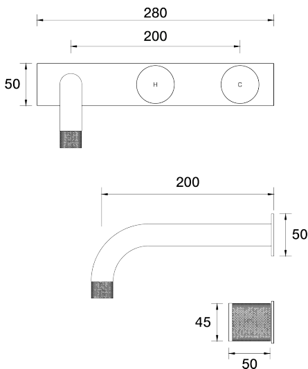
IDK Wall Basin Set Outlet 200mm on Plate - Offset B38.152.6.01 - Chrome
