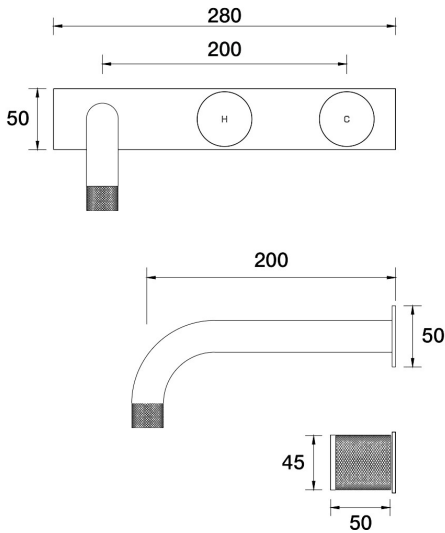
IDK Wall Basin Set Outlet 200mm on Plate - Offset B38.152.6.40 - Rumbled Brass
