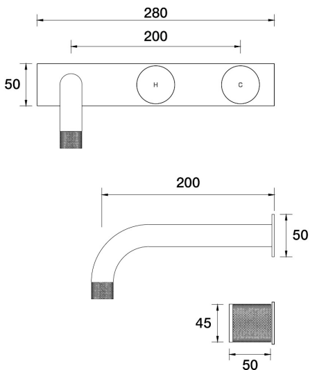
IDK Wall Basin Set Outlet 200mm on Plate - Offset B38.152.6.43 - Brass
