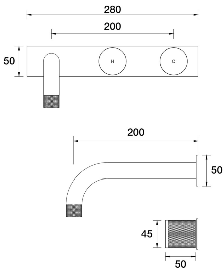
IDK Wall Basin Set Outlet 200mm on Plate - Offset B38.152.6.57 - Matt Nickel
