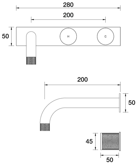
IDK Wall Basin Set Outlet 200mm on Plate - Offset B38.152.6.70 - Sea Spray
