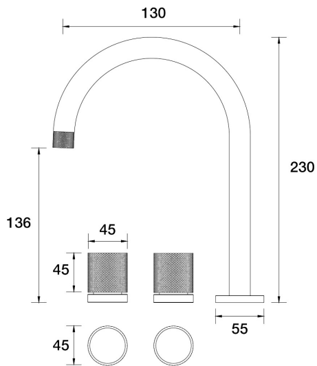
IDK Marble Basin Set Swivel Bianco Marble B39.011.1.34 - Matt Black
