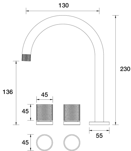
IDK Marble Basin Set Swivel Nero Marble B39.011.2.02 - Brushed Chrome
