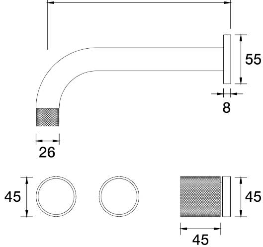
IDK Marble Wall Bath Set 160mm Outlet Nero 160.01.2.01 - Chrome
