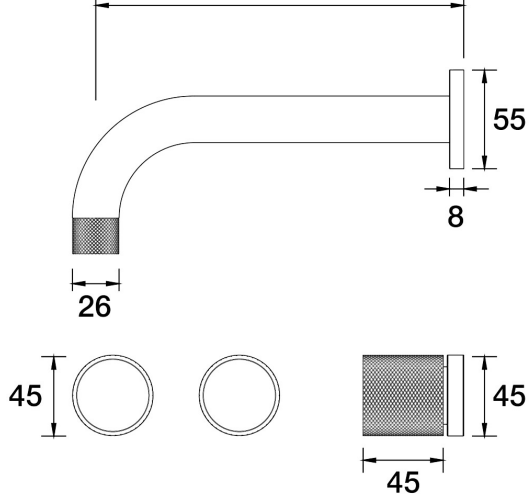
IDK Marble Wall Bath Set 160mm Outlet Nero B99.021.2.57 - Matt Nickel
