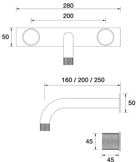
IDK Marble Wall Bath Set 160mm Outlet Nero Marble on Plate B39.021.4.39 - Antique Bronze
