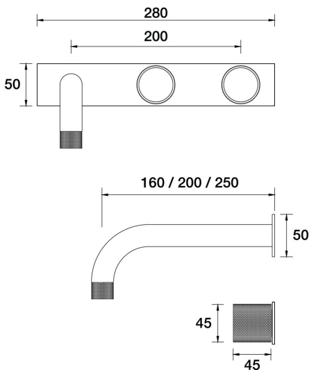
IDK Marble Wall Bath Set 160mm Outlet Bianco Marble on Plate - Offset B39.021.5.01 - Chrome
