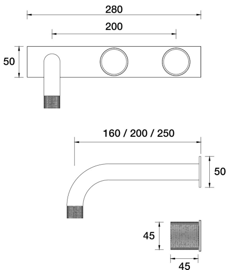
IDK Marble Wall Bath Set 160mm Outlet Bianco Marble on Plate - Offset B39.021.5.75 - Forest Mist
