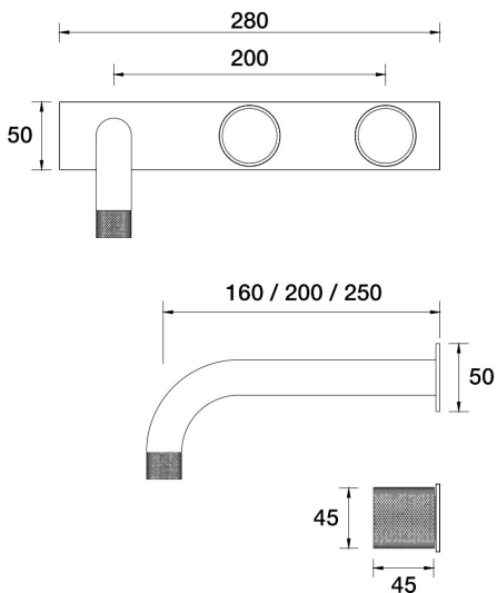
IDK Marble Wall Bath Set 160mm Outlet Nero Marble on Plate - Offset B39.021.6.54 - Volcanic Grey
