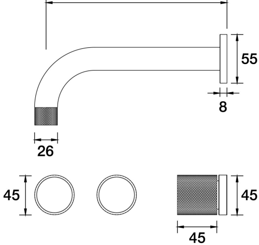
IDK Marble Wall Bath Set 200mm Outlet Bianco Marble
